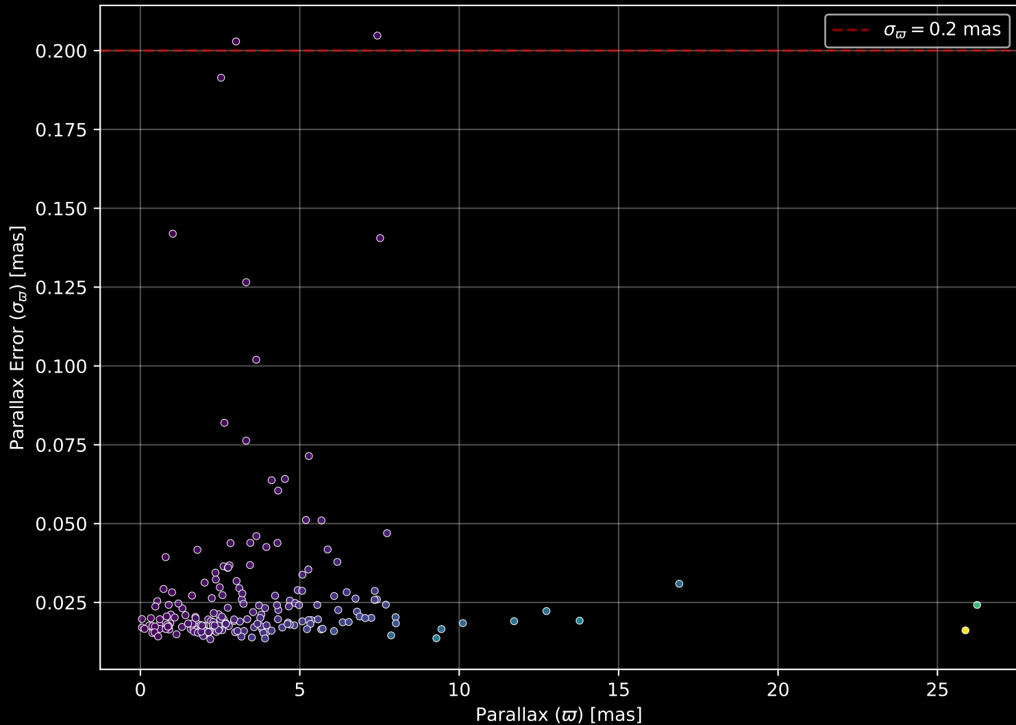
APOGEE DR17 Field: [319+88_MGA] Parallax Quality (n= 200)
