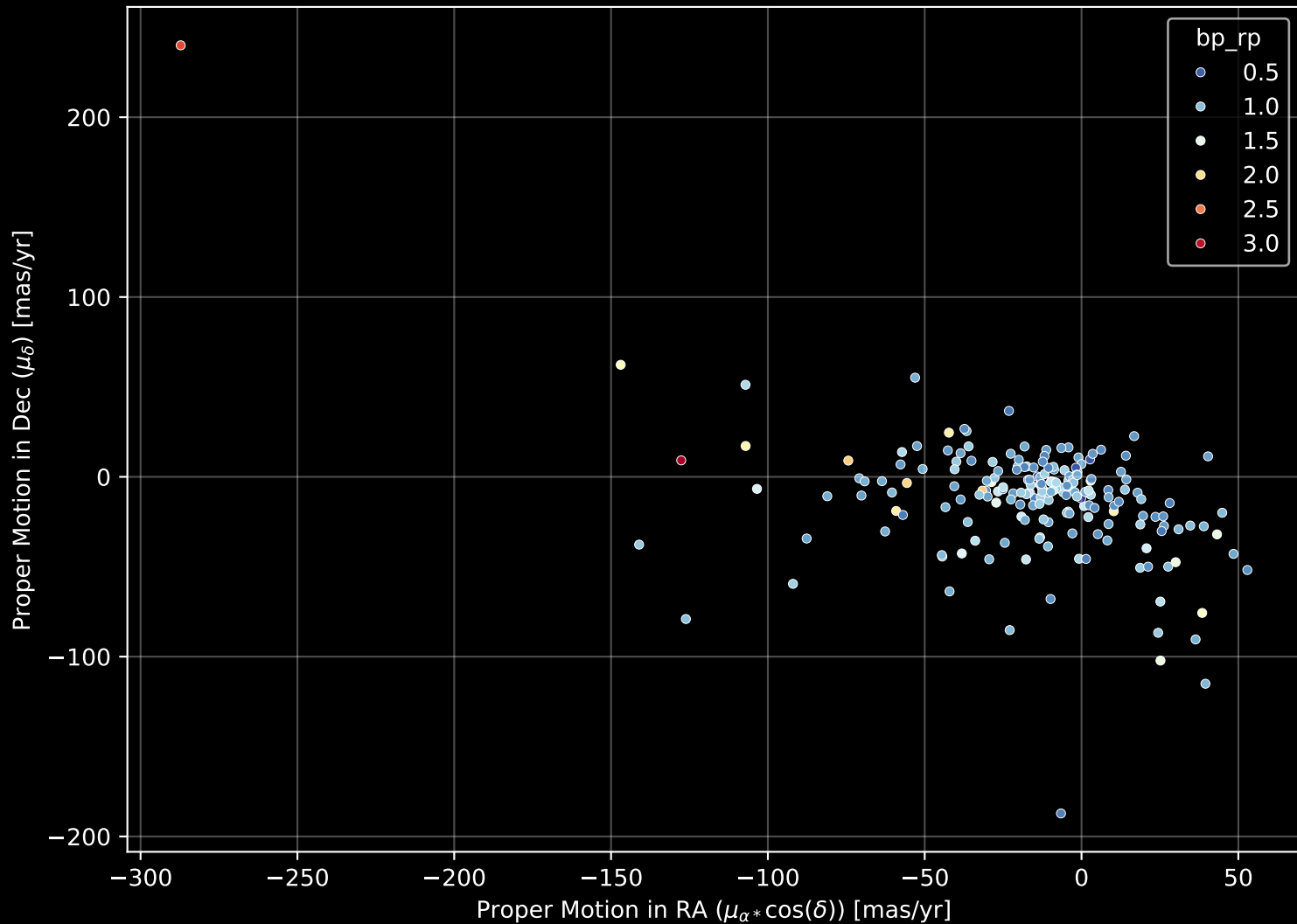
APOGEE DR17 Field: [319+88_MGA] Proper Motion Diagram (n= 200)
