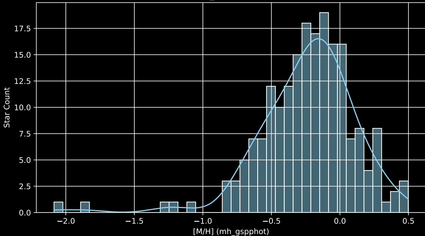
APOGEE DR17 Field: [319+88_MGA [M/H] (mh_gspphot) (n= 198)
