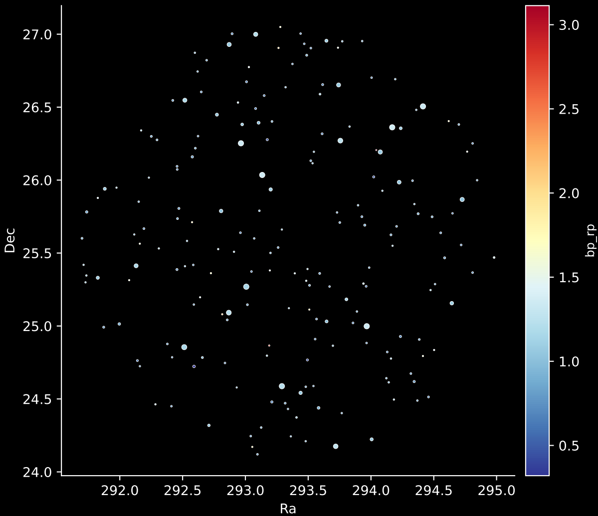
APOGEE DR17 Field: [319+88_MGA] Stars: 200
