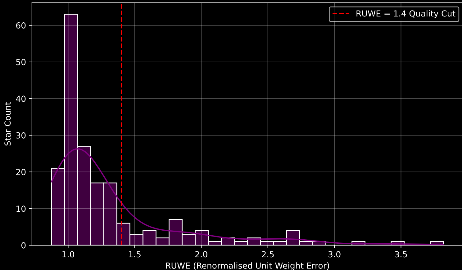
GAPOGEE DR17 Field [319+88_MGA] RUWE Distribution (n= 191)
