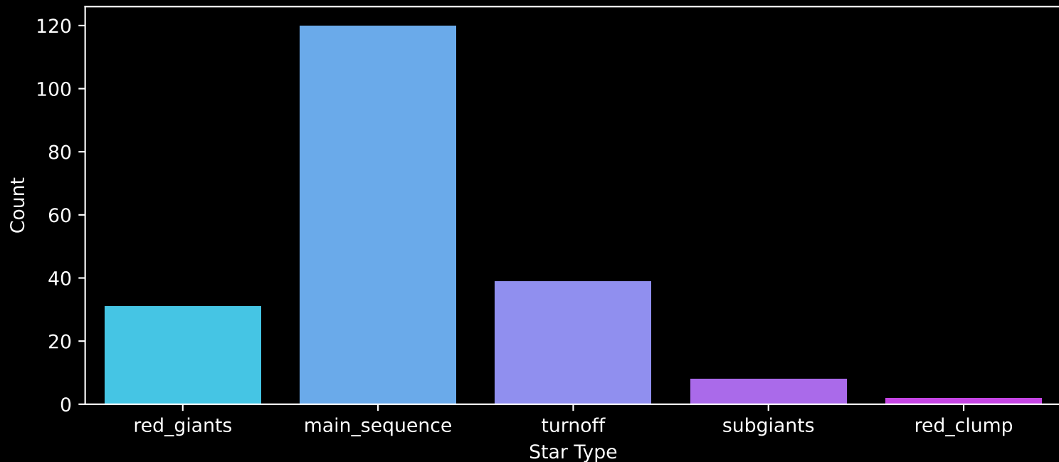
APOGEE DR17 Field: [319+88_MGA] Count plot of Star Type
